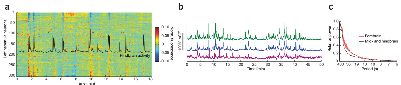
Figure 4 | Single-neuron activity in the left habenula and correlation to hindbrain activity. (a) Activity traces of all neurons in a manually segmented habenula. Habenula neuron activity traces are ordered by correlation coefficient to average hindbrain activity (black trace), with negative correlations at the top and positive correlations at the bottom. Populations that are both strongly positively correlated and negatively correlated are present, as are neurons with ongoing, uncorrelated activity. (b) Three examples of activity traces of habenula neurons. Single-neuron activity is ongoing, with fluctuations on timescales of ~10–30 s, and can in addition be modulated on timescales of minutes, switching between ongoing activity and apparent quiescence. (c) Power spectra of \Delta F/F signals from all supervoxels in the forebrain and all supervoxels in the mid- and hindbrain. Shaded regions show standard error. Data were normalized to the average mid- and hindbrain power spectra, so that the black line does not carry error bars (for a_i and b_i being the forebrain and midbrain/hindbrain power spectra for fish i , respectively, and b_{\text{avg}} the average of all b_i , plotted are b_{\text{avg}} (black) and a_i \times b_{\text{avg}} / b_i (red, mean \pm s.d.)). Relative power in the forebrain is enhanced on timescales between 10 s and several minutes.
