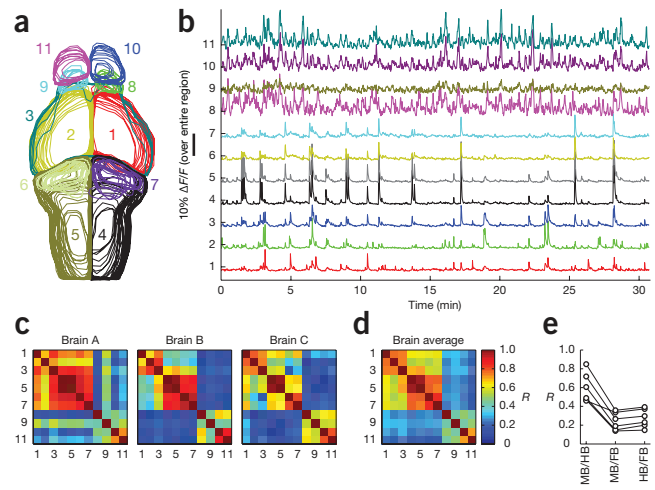
Figure 3 | Correlations and activity patterns across brain regions. (a) Manual segmentation of brain regions. 1,2: right and left midbrain; 3: ventral midbrain; 4,5: right and left hindbrain; 6,7: cerebellum; 8,9: habenula; 10,11: pallium. (b) Fluorescence ( \Delta F/F ) traces in each brain area of a in a transgenic fish expressing GCaMP5G in almost all neurons ( elavl3:GCaMP5G ). Hindbrain areas (4–7) are often activated together, and midbrain activation (1–3) sometimes co-occurs with hindbrain activation. Forebrain activity is qualitatively distinct, characterized by ongoing activity, at long timescales (on the order of 10 s). Average forebrain activity is not clearly coactivated with mid- and hindbrain activity. (c) Correlation matrices of brain area activity for three fish (Brains A, B and C); numbering as in a . Mid- and hindbrain activity are self-correlated and correlated to each other; activity in forebrain areas is self-correlated; and average forebrain activity appears weakly correlated to mid- and hindbrain activity. Note that zero correlation for activity averaged over brain areas does not necessarily imply the absence of correlations on the single-neuron level (see Fig. 4 ) and that correlational structure reflects activity in the particular experimental conditions used to derive these data. (d) Average correlation coefficients ( R ) of six fish. (e) Correlations between the entire hindbrain (HB), midbrain (MB) and forebrain (FB) for six fish.
