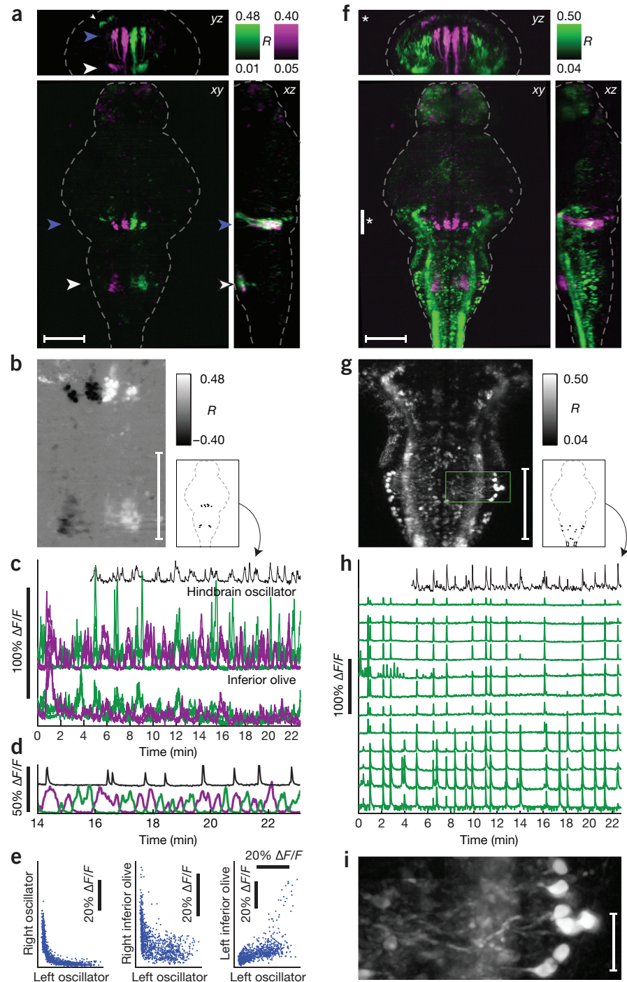
Figure 6 | Whole-brain, neuron-level identification of two functionally defined circuits. (a) Maximum-intensity projection of voxels positively (green) and negatively (magenta) correlated to the reference trace (black trace in c ). Top, front projection. Bottom, top projection. Right, side projection. The hindbrain oscillator appears at single-neuron resolution in the anterior hindbrain (caudal to cerebellum; blue arrowheads). In addition, the inferior olive (white arrowheads) exhibits ipsilateral correlations to the hindbrain oscillator. (b) Enlarged view of hindbrain oscillator and inferior olive. (c) Functional GCaMP5G signals (as change in fluorescence, \Delta F/F ) of ten manually isolated neurons in the hindbrain oscillator and six isolated neurons in the inferior olive, indicated in the map in b . Colors as in a . Reference signal is shown in black (first 4.5 min of data were discarded to avoid transient effects). (d) Average signal of all 16 neurons from c . For comparison, average signal from h is shown in black. The two signals are independent. (e) Scatter plots of left and right average population activity. (f) Spinal-hindbrain network, in the same fish, derived from the same time-lapse recording. Magenta, populations from a ; green, correlation to a second functional trace (top trace in h ). The yz projection (asterisk) is based on the volume section indicated by the white bar and asterisk in the xy projection. (g) Enlarged view of the spinal-hindbrain population. (h) Functional GCaMP5G signals in selected neurons of the spinal-hindbrain population and from two patches of neuropil in the spinal cord (top two traces). Reference signal is shown in black. (i) Detail of g showing neurites. Gamma was adjusted to aid visualization. Scale bars, 100 \mu\text{m} ( a,b,f,g ), 20 \mu\text{m} ( i ).
